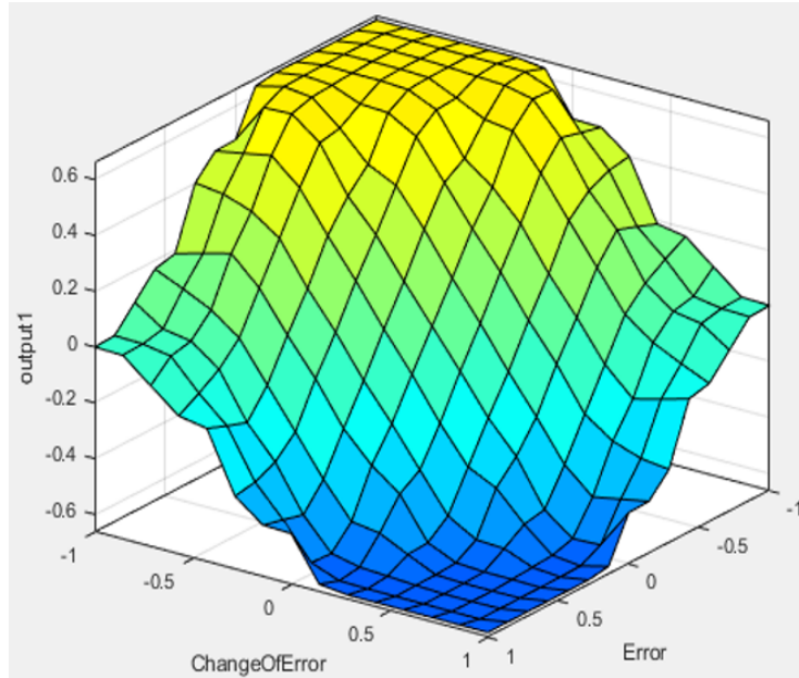
Figure 4. Fuzzy surface of 5x5 fuzzy Mamdani membership rules
