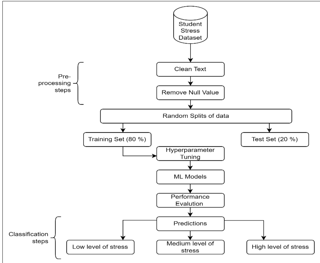
Figure 3 Proposed Methodology
