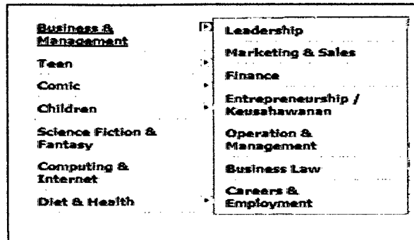
Figure 10: Category Part
