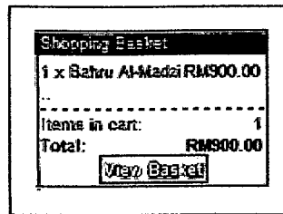
Figure 6: Shopping Basket
