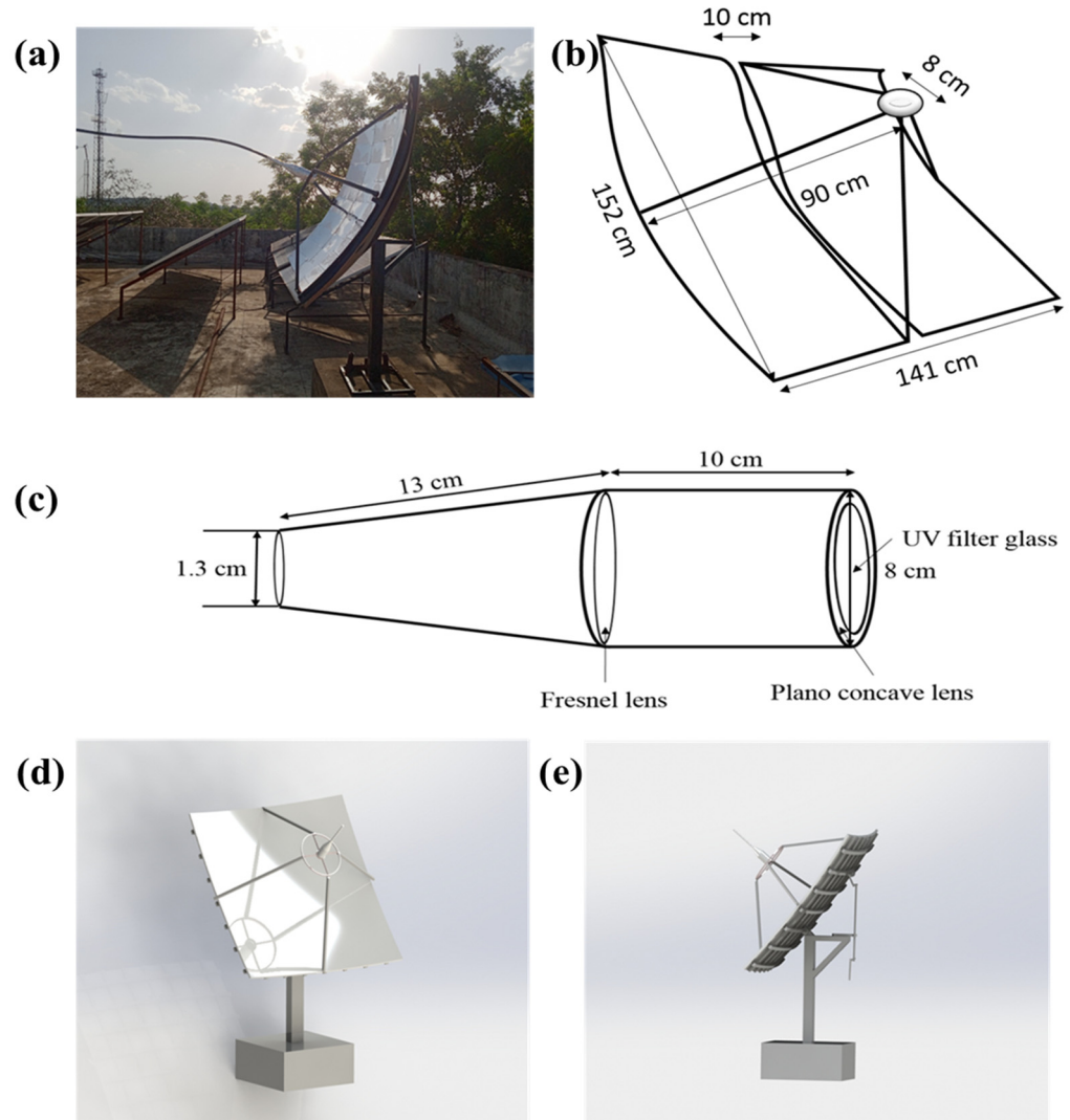
Figure 1. (a) Installed solar daylighting system on the roof of an energy center. (b) Dimensions of the installed apparatus. (c) Receiver cavity. (d,e) Three-dimensional drawings of the design.
