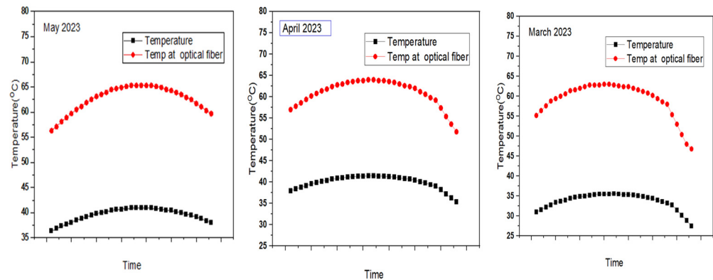
Figure 3. Temperature comparison of ambient vs. internal at optical fiber for different months.
