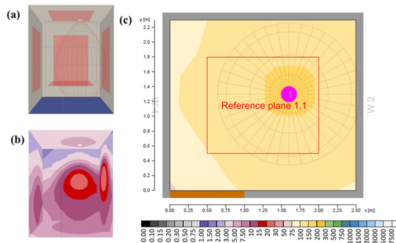
Figure 5. Simulation results: (a) 3D view of the demo room, (b) pseudo-color model showing light distribution (lux), and (c) pseudo-reference plane.
