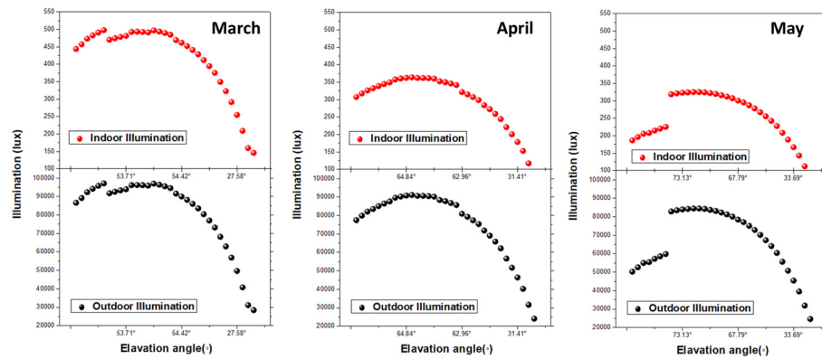
Figure 4. Illumination comparison ambient vs. indoor at optical fiber for different months.
