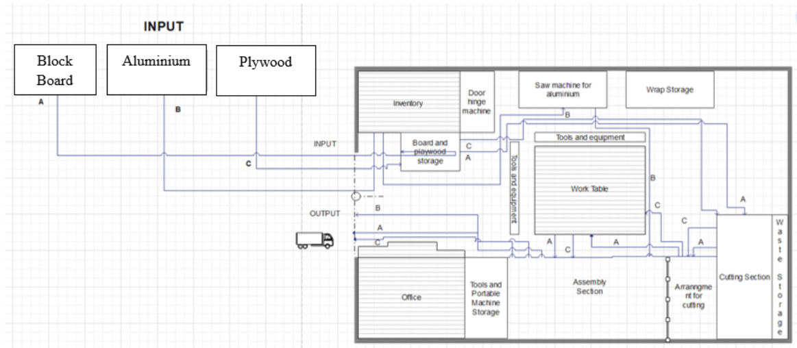
Figure 2. Plant layout
