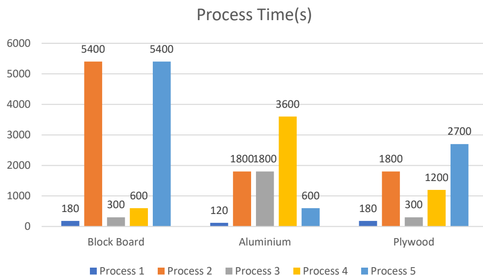
Figure 7. Process time
