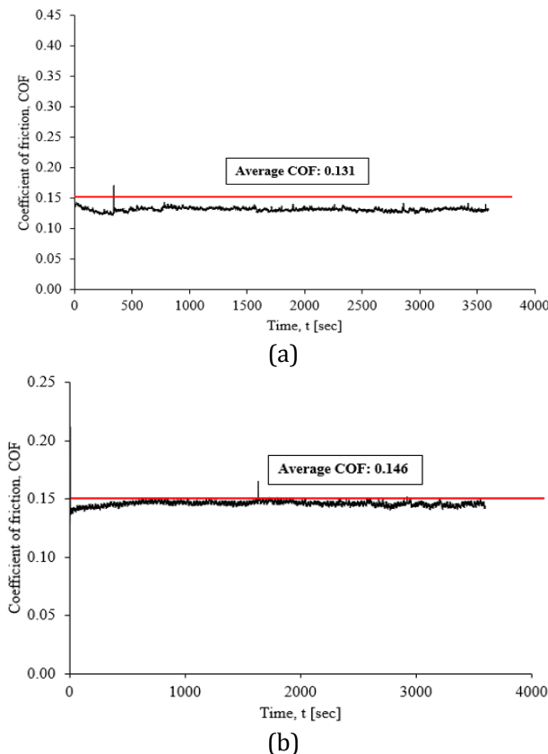
Figure 4: (a) Coefficient of friction, COF vs time, t graph of tribology result with nanoparticles ( \text{SiO}_2 ) (b) Coefficient of friction, COF vs time, t graph of tribology result without nanoparticles.
