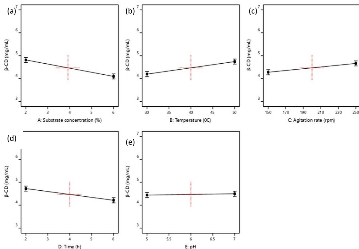
Fig. 1. Plot of the effect of (a) Substrate concentration (2 – 6%) (b) Temperature (30 – 50 ^{\circ}\text{C} ) (c) Agitation rate (150 – 250 rpm) (d) time (2 – 6 h) (e) pH (pH 5 - 7) on the \beta -CD production from the immobilization of E. coli on hollow fiber membrane
