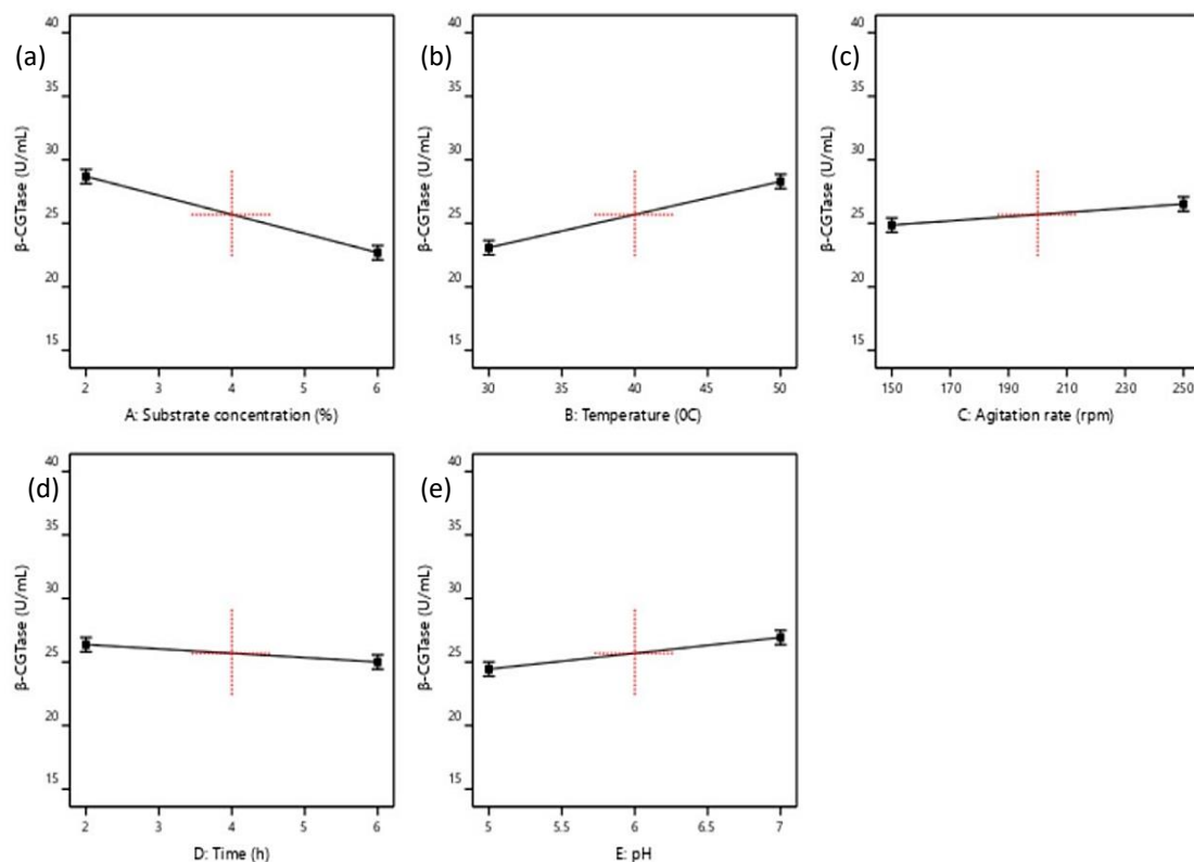
Fig. 2. Plot of the effect of (a) Substrate concentration (2 – 6%) (b) Temperature (30 – 50 ^{\circ}\text{C} ) (c) Agitation rate (150 – 250 rpm) (d) time (2 – 6 hr) (e) pH (pH 5 - 7) on the \beta -CGTase excretion from the immobilization of E. coli on hollow fiber membrane
