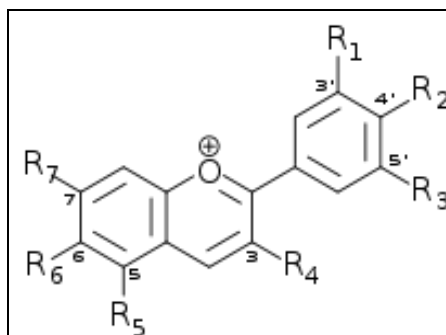
Figure 2.1 The flavylum ion. (Francis et al. , 2000)
