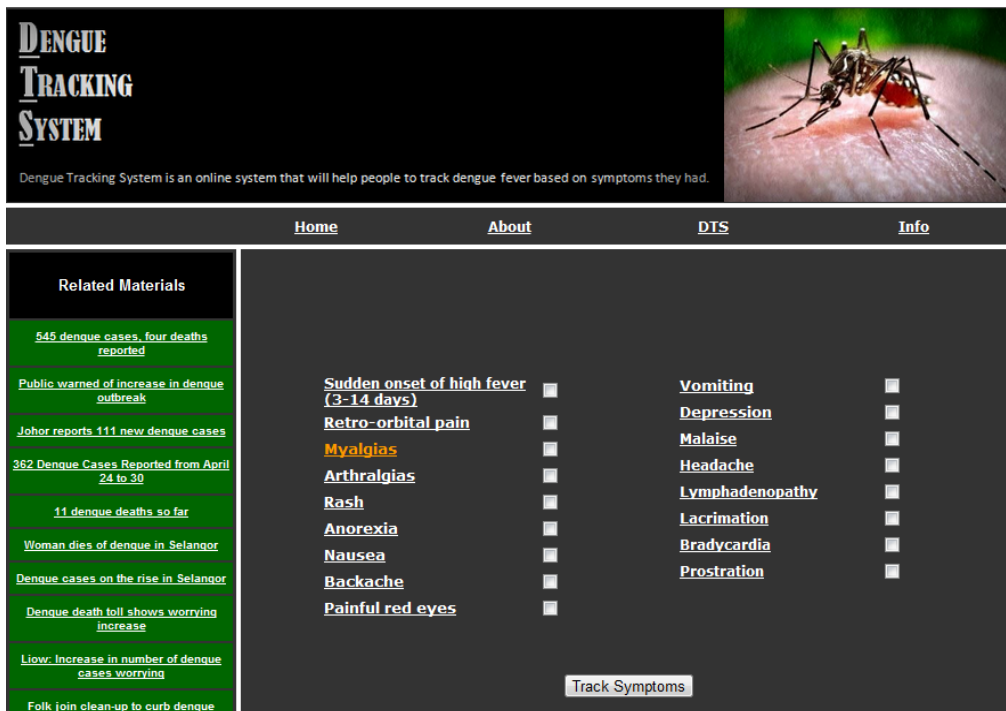
Figure 3.3: Symptom's link
