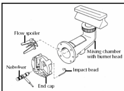
Figure 2.5: Typical Burner and Spray Chamber
