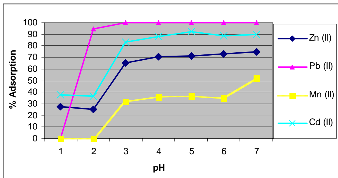
Figure 4.3: Removal of Some Metal Ion on the H + -form SOW as a Function of Equilibrium pH. Weight of the Gel = 0.1 g. Volume of the Simulated Waste Water = 60 ml. Initial Metal Concentration = 5 ppm
