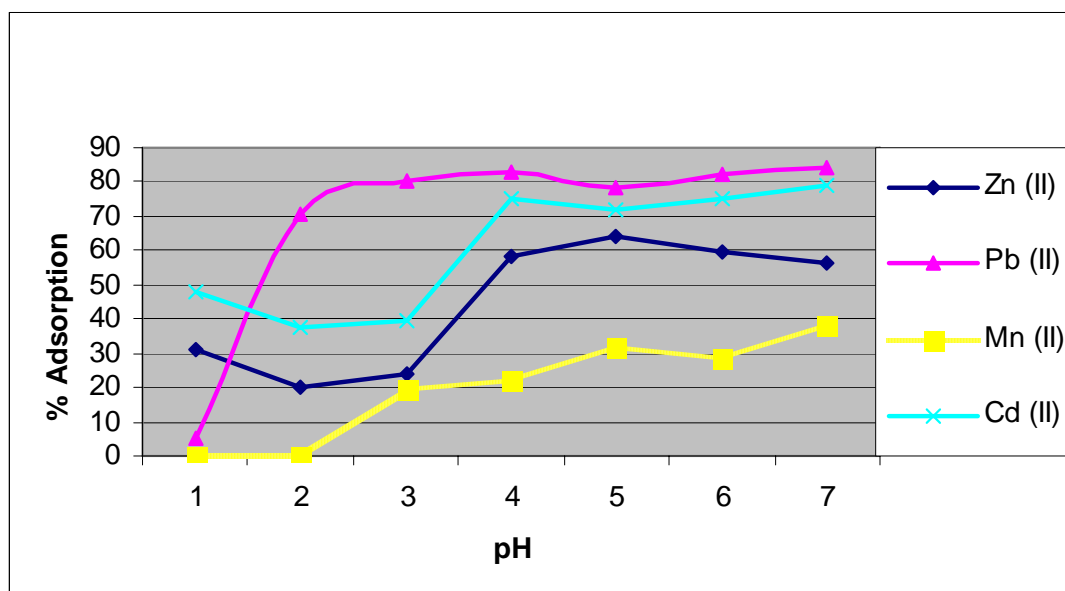
Figure 4.2: Removal of Some Metal Ion on the \text{Ca}^{2+} -form SOW as a Function of Equilibrium pH. Weight of the Gel = 0.1 g. Volume of the Simulated Waste Water = 60 ml. Initial Metal Concentration = 5 ppm
