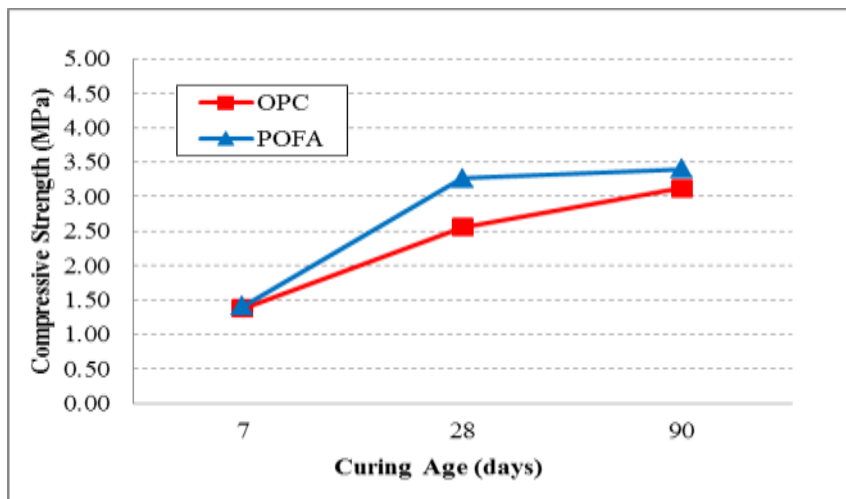
Fig. 5: Compressive strength development of aerated concrete mixes at the age of 7, 28 and 90 days
