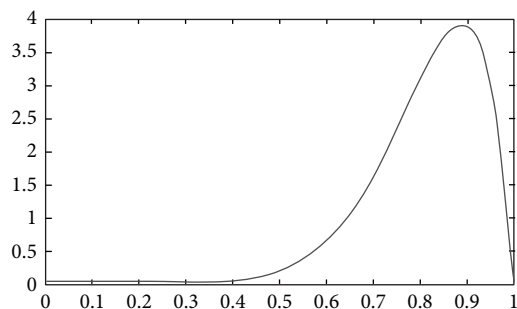
FIGURE 1: A beta distribution with \alpha = 9 and \beta = 2 .
