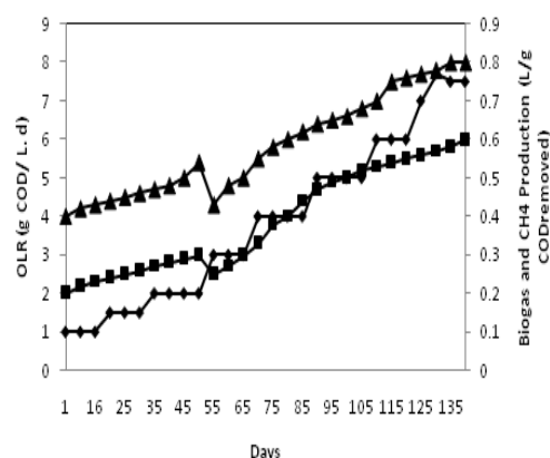
Figure 2: Biogas and CH 4 production in terms of OLR influence, where ♦ OLR (g COD/L), ■ CH 4 production (L/g COD removed ), ▲ Biogas production (L/g COD removed ).
