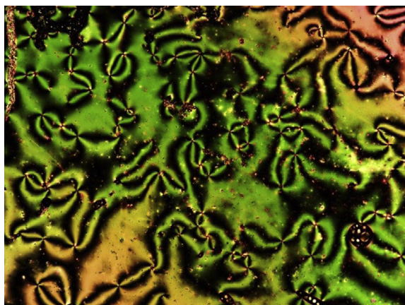
Fig. 2. Polarized optical micrographs obtained from cooling of isotropic phases showing schlieren texture observed for compound 'IVb' at 202.4\text{ }^{\circ}\text{C} on cooling from isotropic melt.
