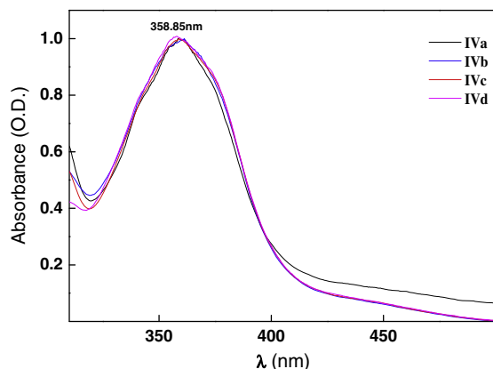
Fig. 3. Absorption spectra before irradiation of the UV light for the compounds IVa–IVd showing similar transition peaks.
