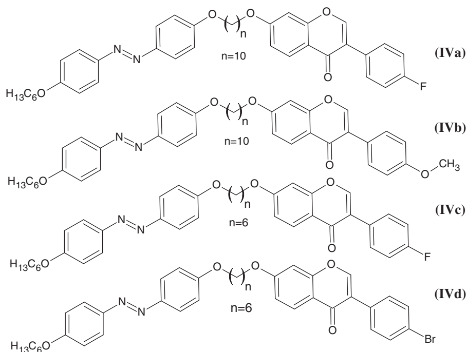
Fig. 1. Chemical structures of the compounds studied in these investigations.
