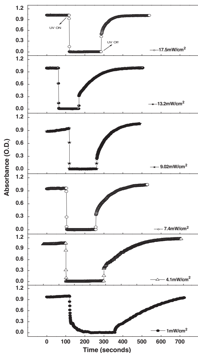
Fig. 8. Z-E photoisomerization of the compounds IVa–IVd. One can see that photo-saturated thermal back relaxation time is around ~90 s for the compound IVc, ~400 s for the compounds IVa and IVb and around 700 s for the compound IVd.
