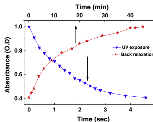
Fig. 9. Behaviour of the compound-IVb with respect to time, in presence of UV light (studied with LC filled cells).
