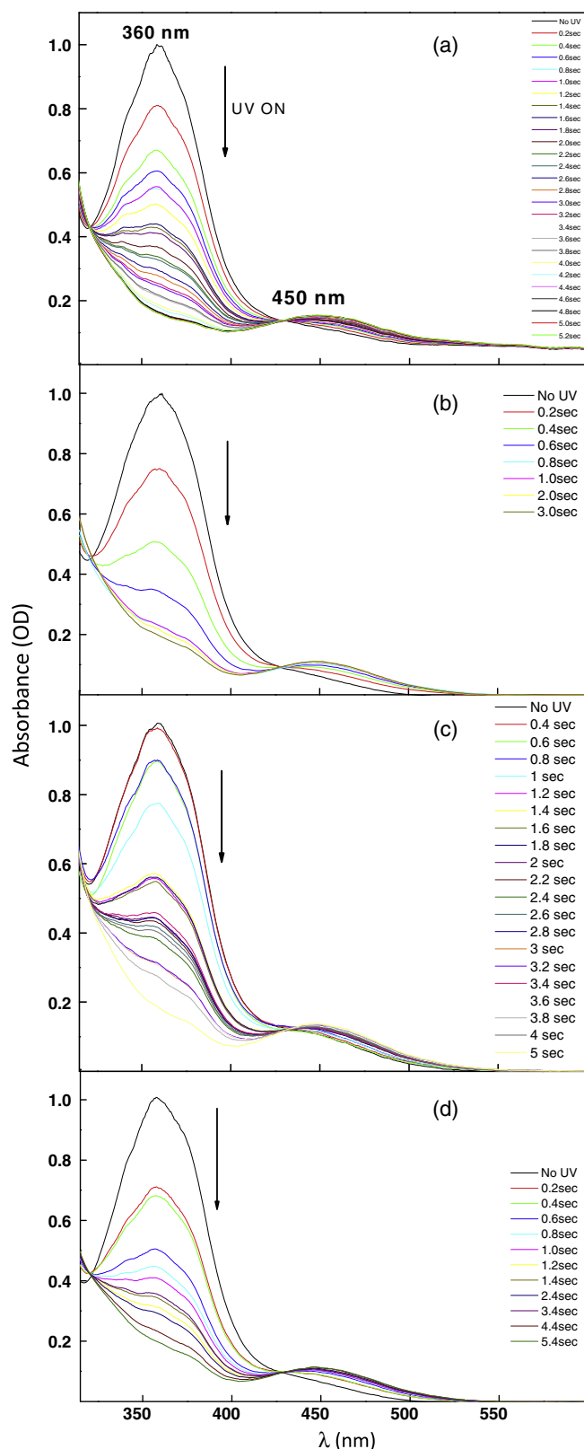
Fig. 4. Showing the absorbance data of all the samples investigated here respectively as IVa–IVd.
