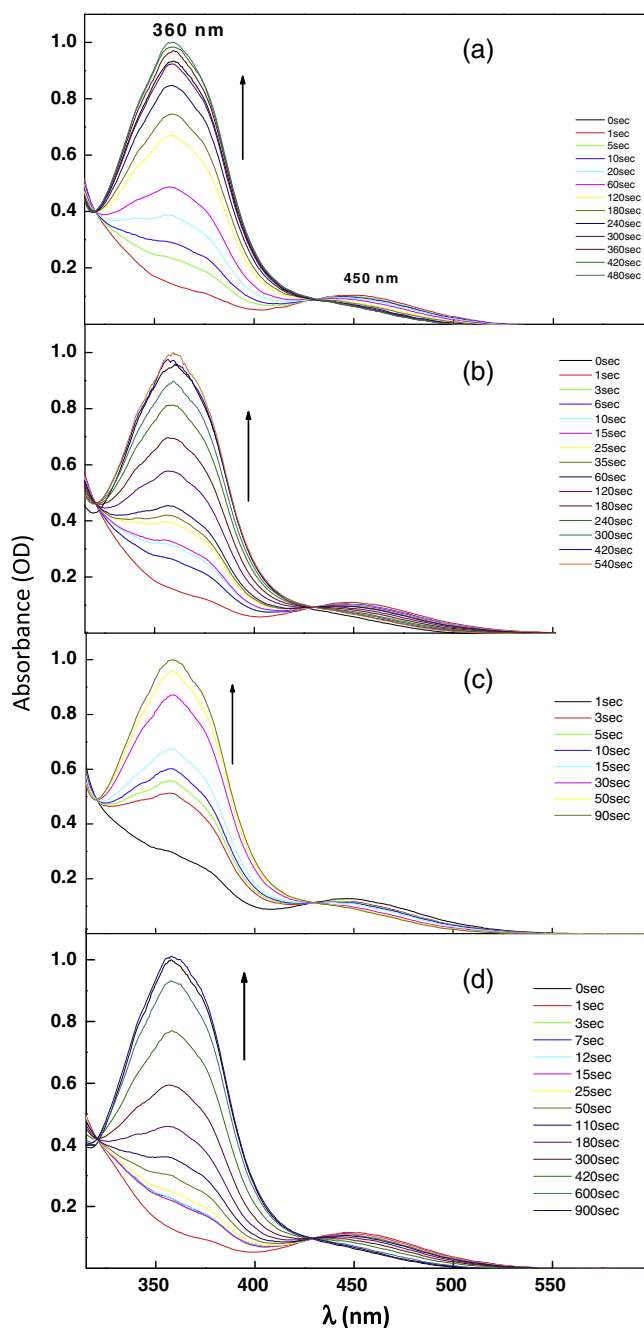
Fig. 6. Showing the thermal back relaxation data of all the samples investigated here namely IV (a), IV (b), IV (c), and IV (d). One can see 2 peaks, one at \sim 365 nm and another at 450 nm.
