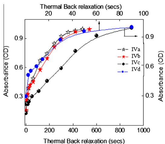
Fig. 7. Thermal back relaxation time for the compound IVb as a function of UV light intensity showing slow back relaxation (lower intensity) to fast thermal back relaxation (higher intensity).
