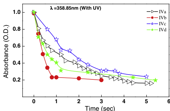
Fig. 5. Showing E–Z isomerization in presence of UV irradiation with respect to exposure time. Data is compared with compounds IVa–IVd respectively.
