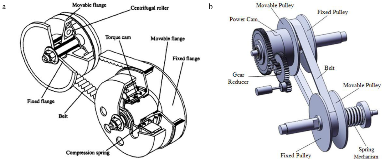
Fig. 2.(a) The conventional of CVT; (b) SAPA.
