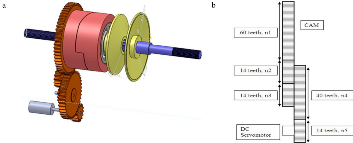
Fig. 4. (a) Gears Reducer; (b) Schematic of gears reducer.
