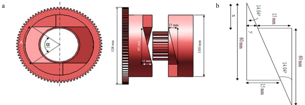
Fig. 5. (a) Power Cam Mechanism; (b) Schematic of power cam mechanism
