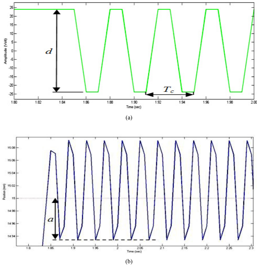
Fig. 6. The results of relay feedback controller (a) Relay output; (b) Waveform of oscillation
