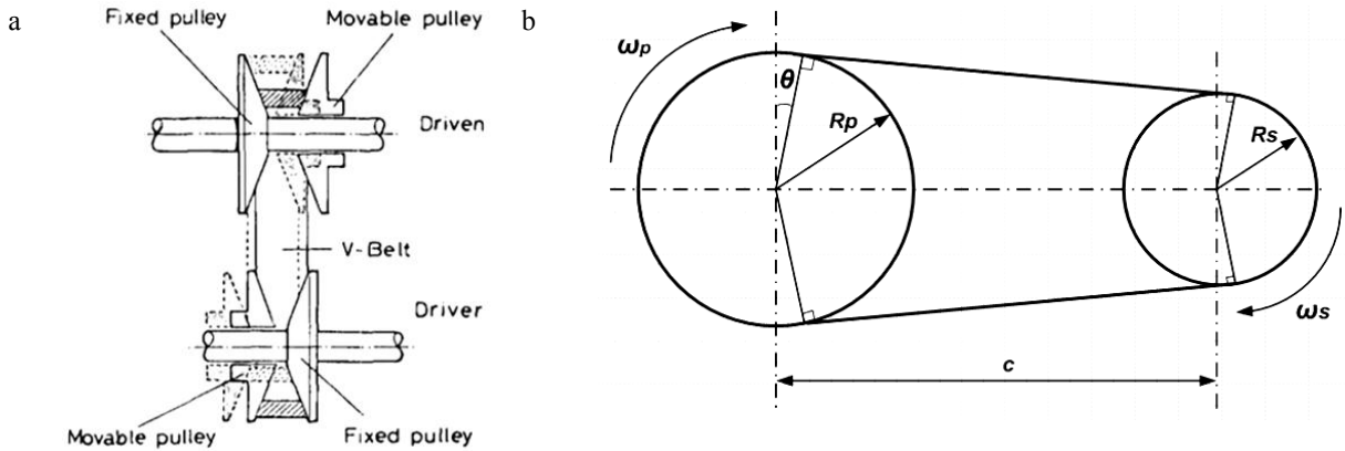
Fig. 1.(a) Principle of a V-belt CVT; (b) Variator geometry.
