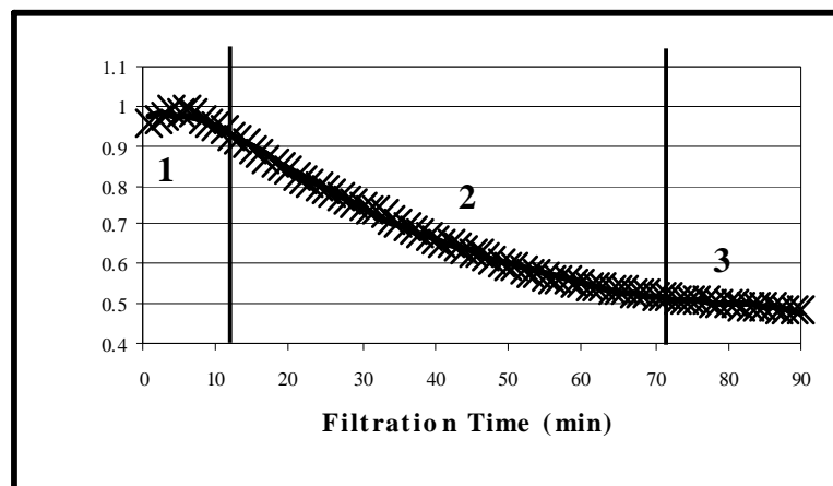
Figure 3.0: Typical curve of filtrate flux versus filtration time in the filtration of Activated Clay from RBD Oil
