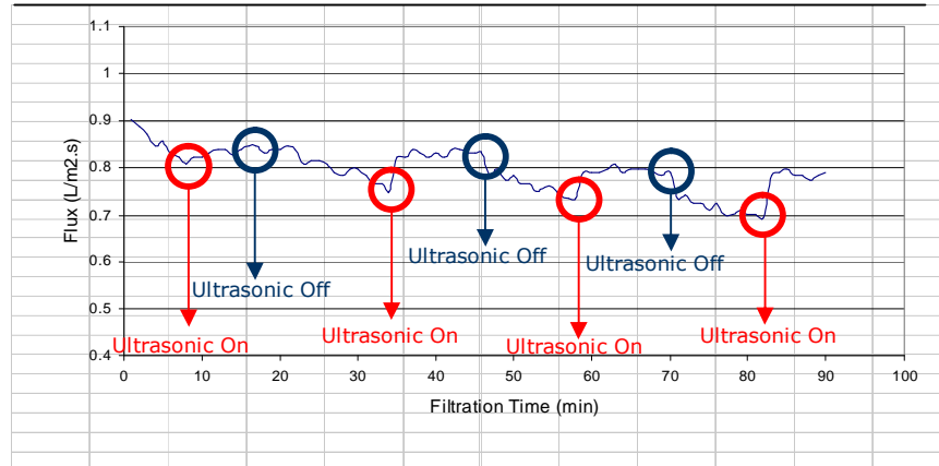
Figure 3.1: Intermittent application of ultrasound field in filtration process
