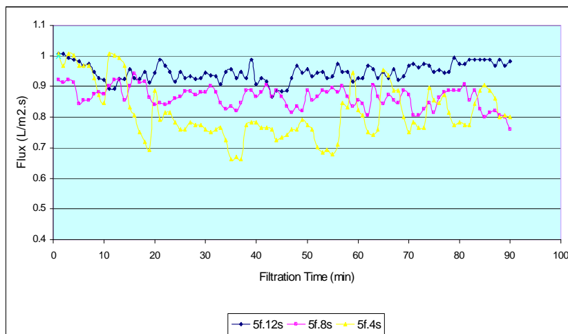
Figure 3.3: Effect of varying the sonication cycle time.\)
