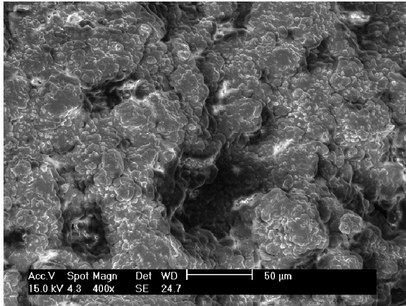
Figure 3.2(b): Scanning electron micrograph (x400) of cake structure after Ultrasonication
