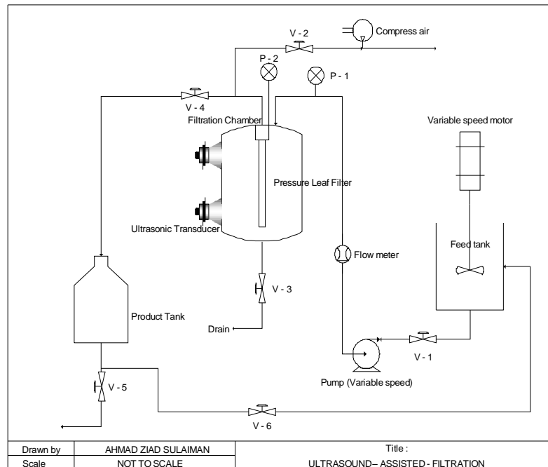
Figure 1.0: Schematic Diagram of the experimental setup for ultrasound-assisted filtration
