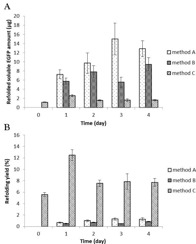
Figure 2. The recovery of refolded soluble EGFP from methods A, B, and C under various refolding incubation periods (dotted, method A; grid, method B; and downward diagonal, method C). (A) Amount of refolded soluble EGFP. (B) Refolding yield of refolded soluble EGFP. Error bars represent duplicate independent experiments with duplicate measurements.
